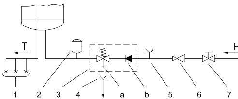
Fig. 3: Closed (pressure) system
