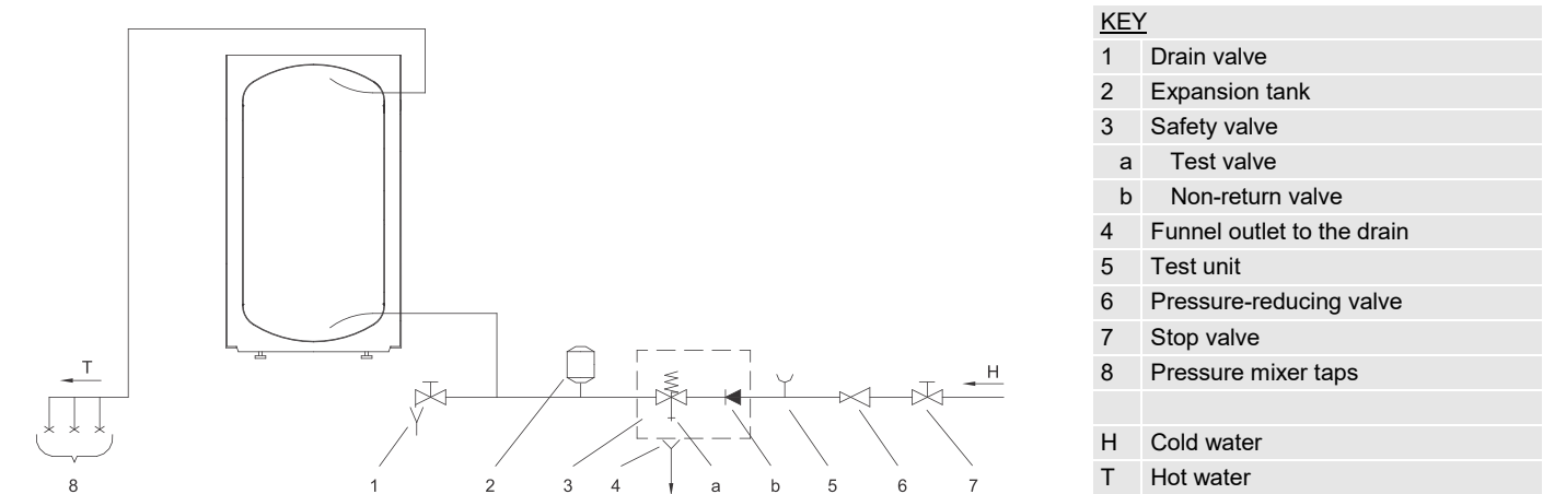
Image 3: Closed (pressure) system
