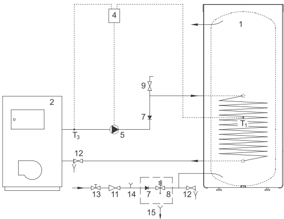
Image 8: Connection to the central heating hot-water system
