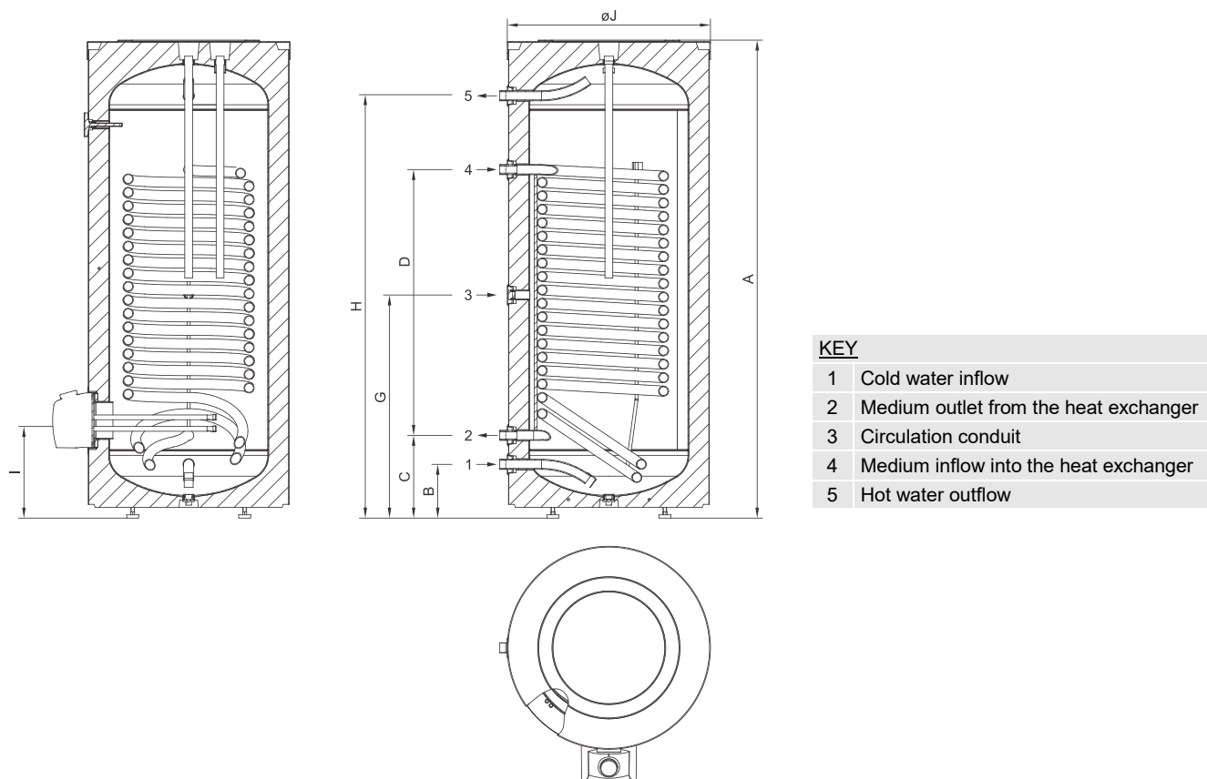
Image 1: Connection and installation dimensions of the storage tank [mm]
