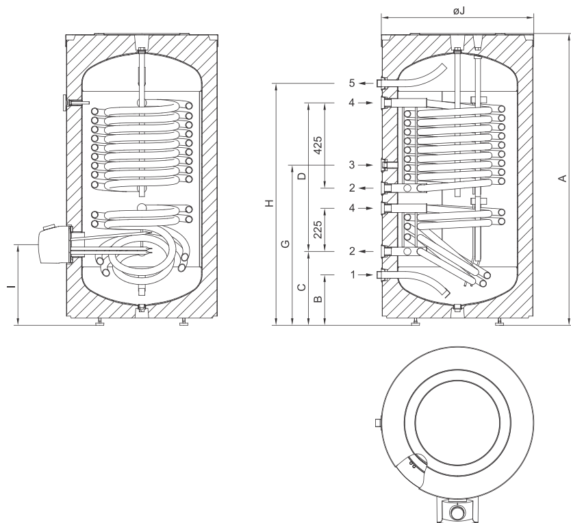
Image 2: Connection and installation dimensions of the storage tank [mm]
