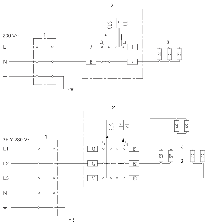
Image 5: Schemes of electric installations
